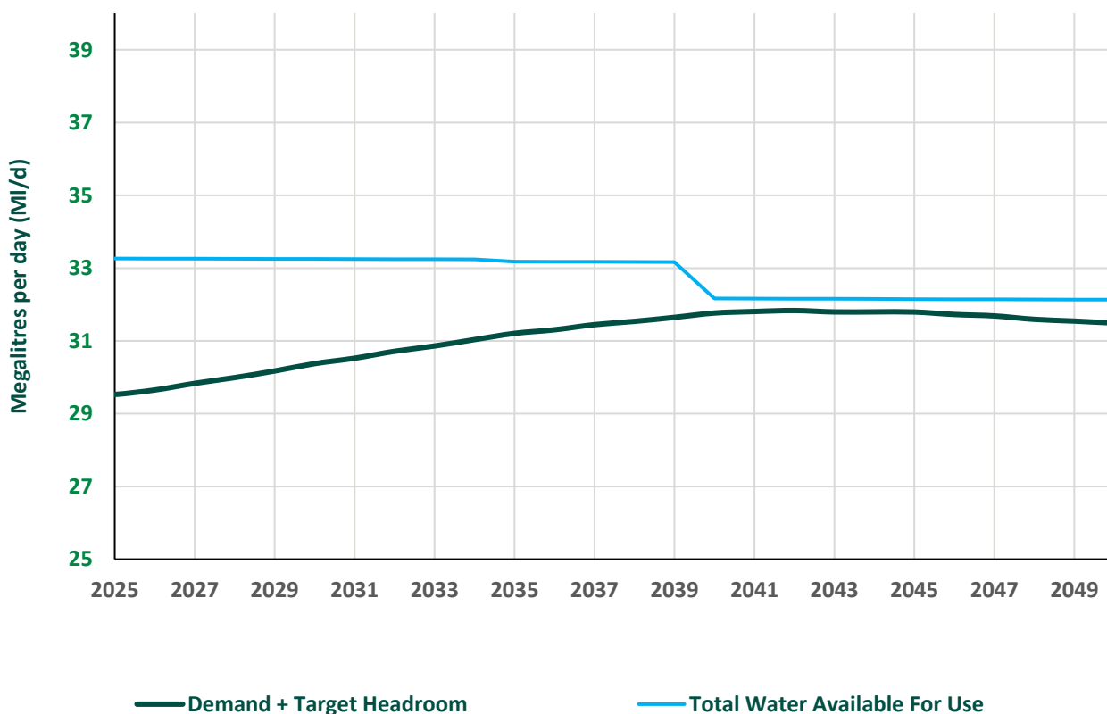
Figure 20 Carlisle Resource Zone – Dry Year Annual Average Supply-Demand Balance
