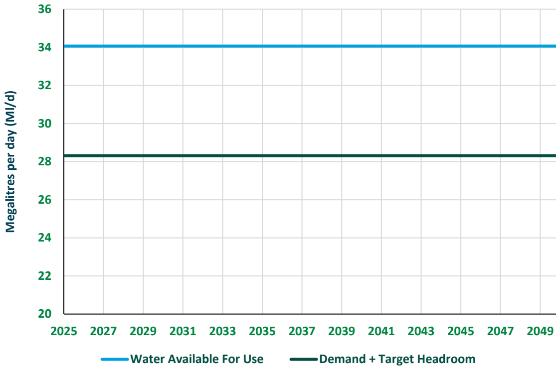
Figure 23 Barepot Resource Zone – Dry Year Annual Average Supply-Demand Balance
