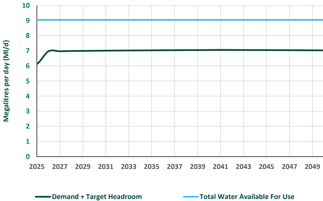
Figure 21 North Eden Resource Zone – Dry Year Annual Average Supply-Demand Balance
